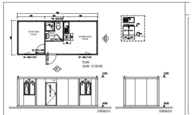
Blueprint of a prefab living
